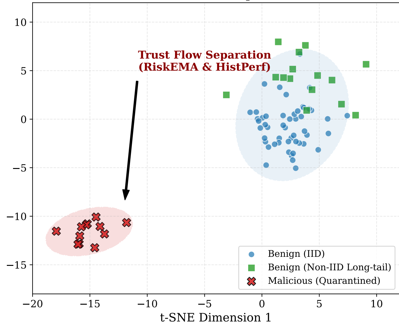
(b) Trust-Flow Defense (Separated Manifold)
