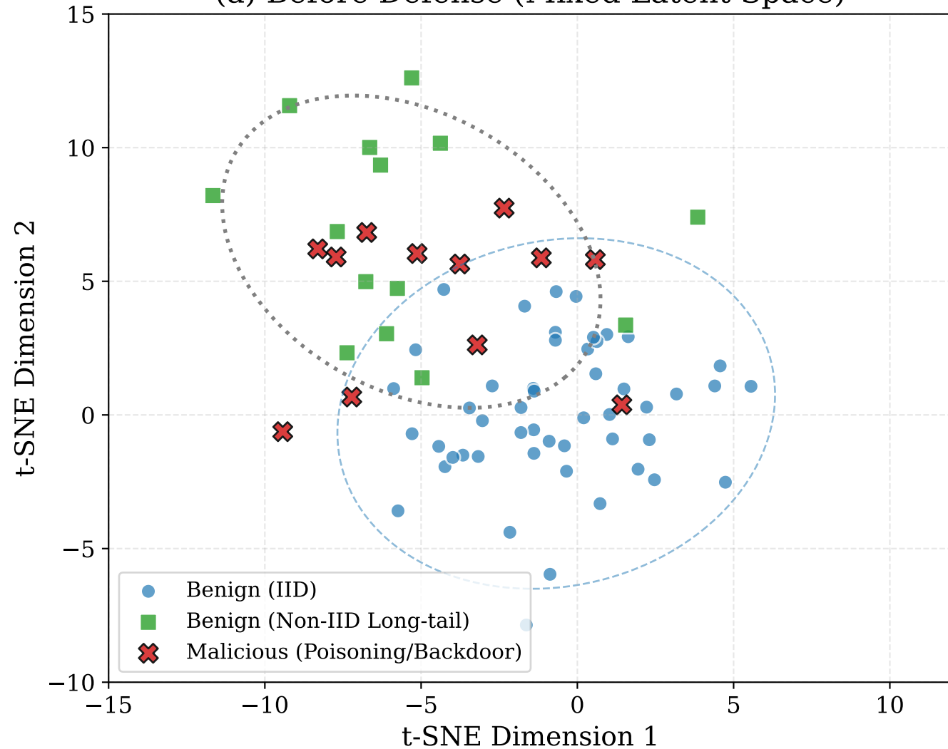
(a) Before Defense (Mixed Latent Space)
